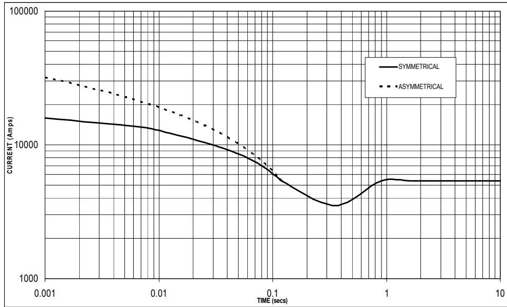
Sustained Short Circuit = 5,400 Amps
