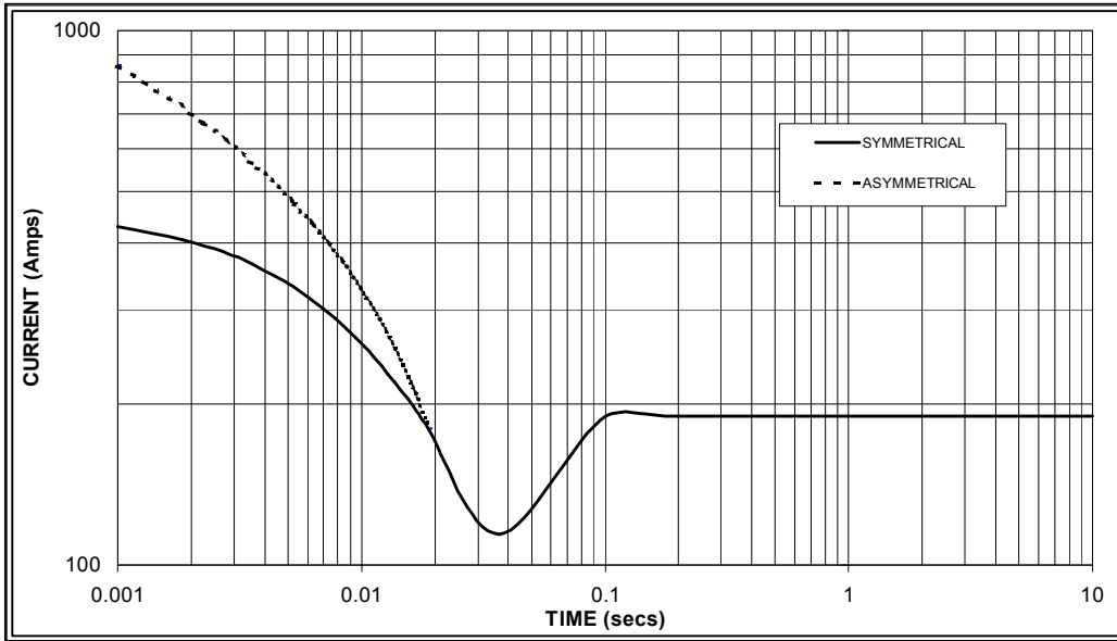
Sustained Short Circuit = 190 Amps
