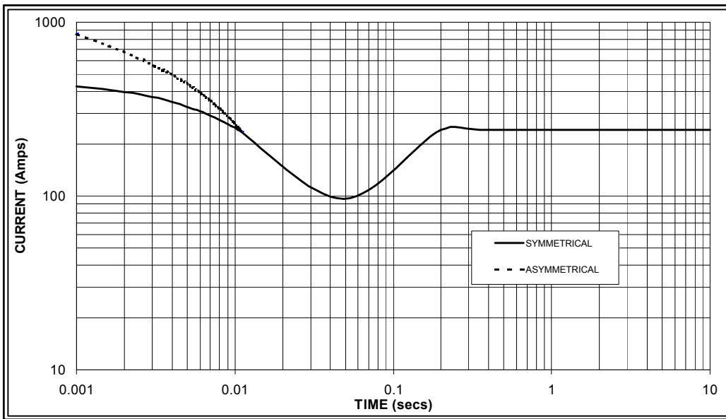
Sustained Short Circuit = 240 Amps
