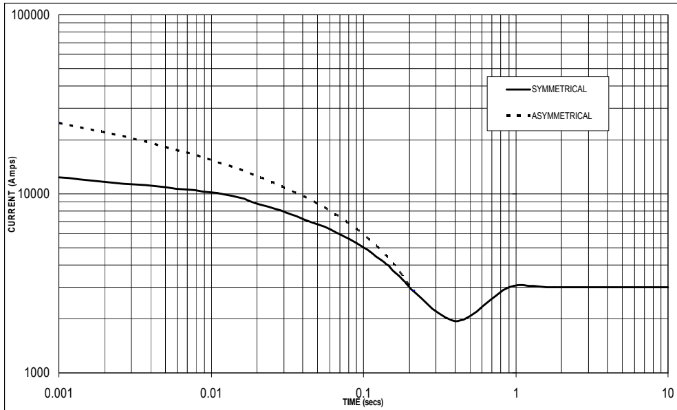
Sustained Short Circuit = 3,000 Amps
