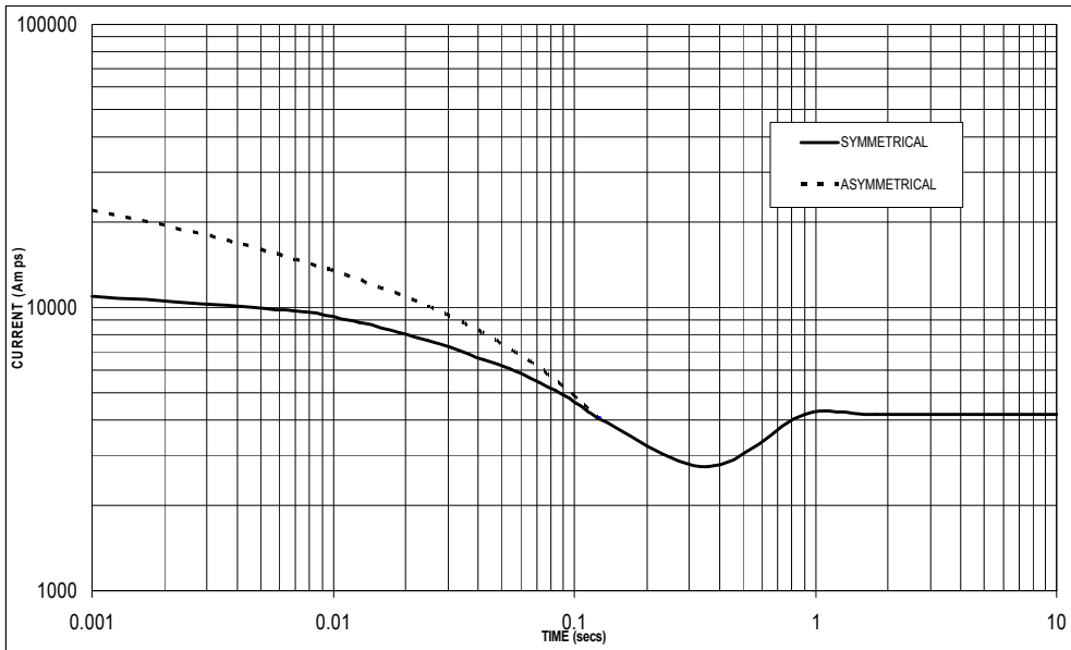
Sustained Short Circuit = 4,200 Amps
