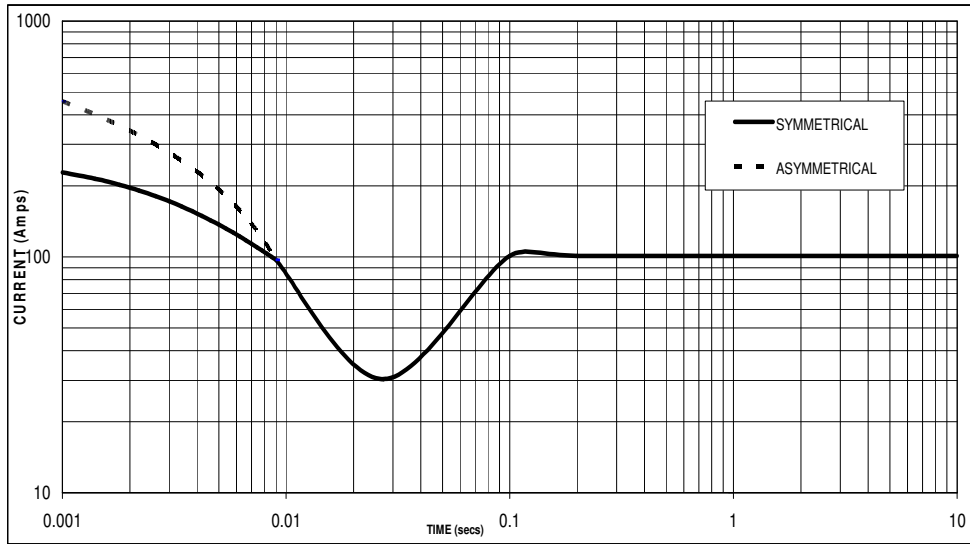
Sustained Short Circuit = 101 Amps
