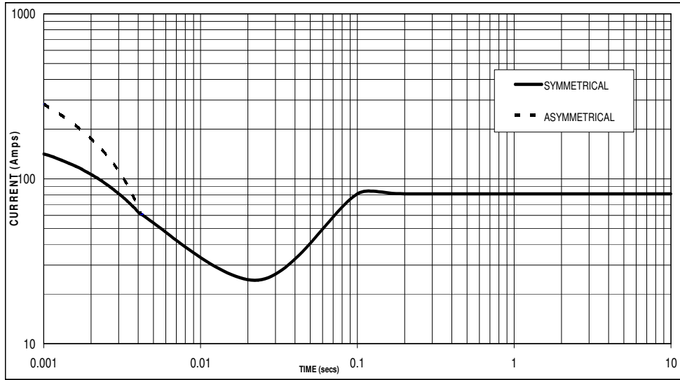
Sustained Short Circuit = 81 Amps
