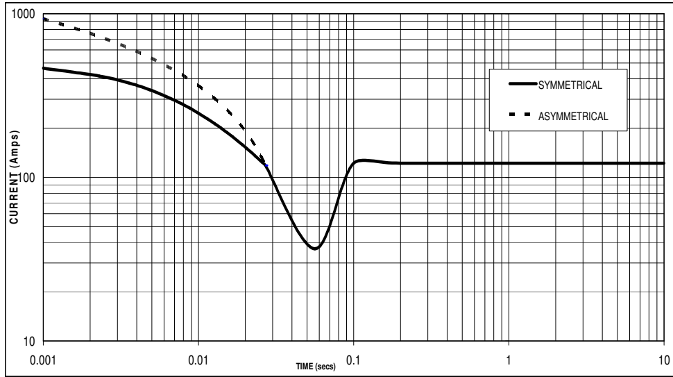
Sustained Short Circuit = 122 Amps
