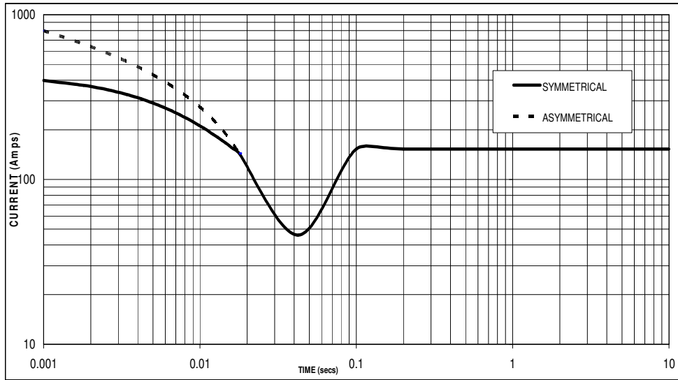
Sustained Short Circuit = 153 Amps
