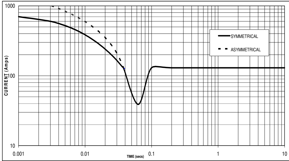
Sustained Short Circuit = 130 Amps
