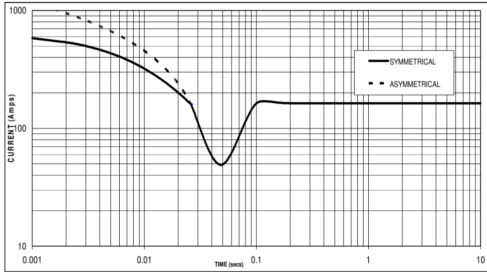
Sustained Short Circuit = 163 Amps
