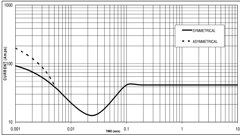
Sustained Short Circuit = 43 Amps
