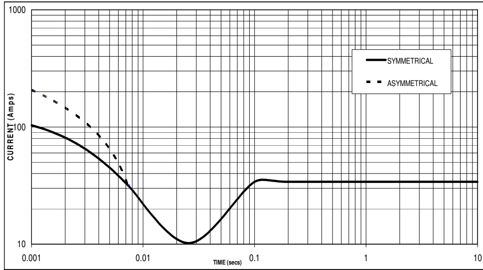
Sustained Short Circuit = 34 Amps
