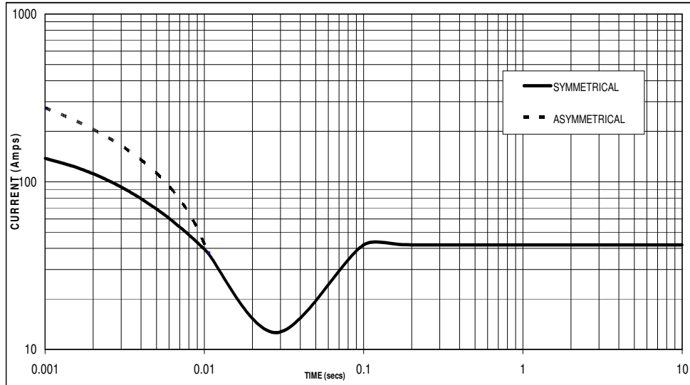
Sustained Short Circuit = 42 Amps
