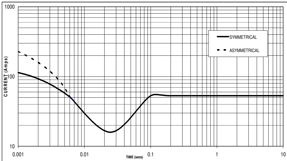
Sustained Short Circuit = 53 Amps
