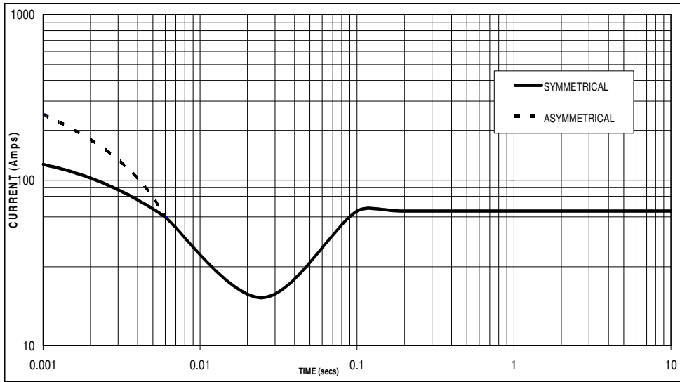
Sustained Short Circuit = 65 Amps
