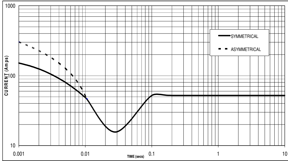
Sustained Short Circuit = 52 Amps
