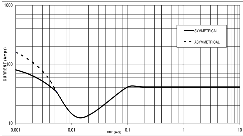
Sustained Short Circuit = 41 Amps
