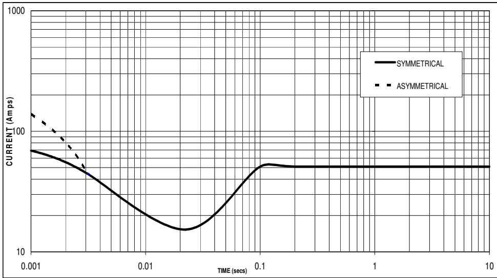
Sustained Short Circuit = 51 Amps
