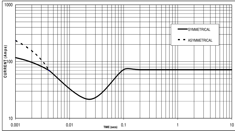
Sustained Short Circuit = 72 Amps
