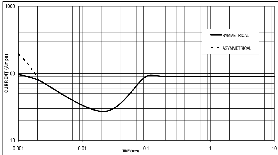
Sustained Short Circuit = 90 Amps
