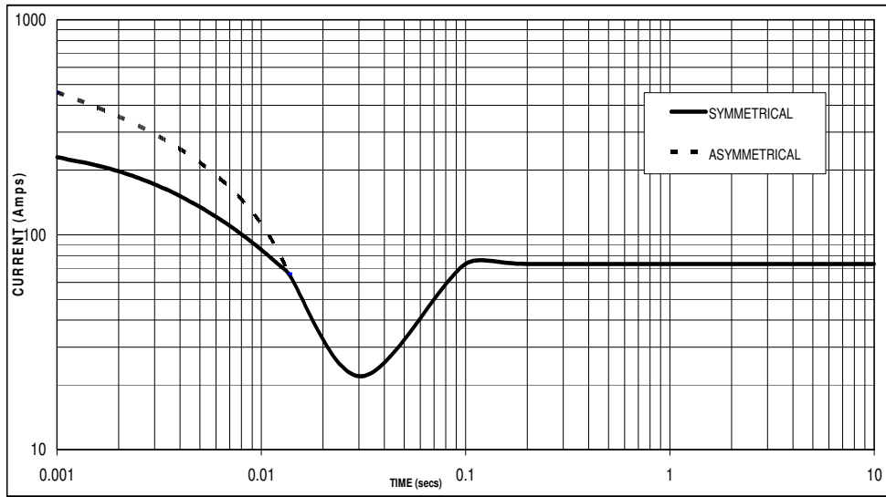
Sustained Short Circuit = 73 Amps
