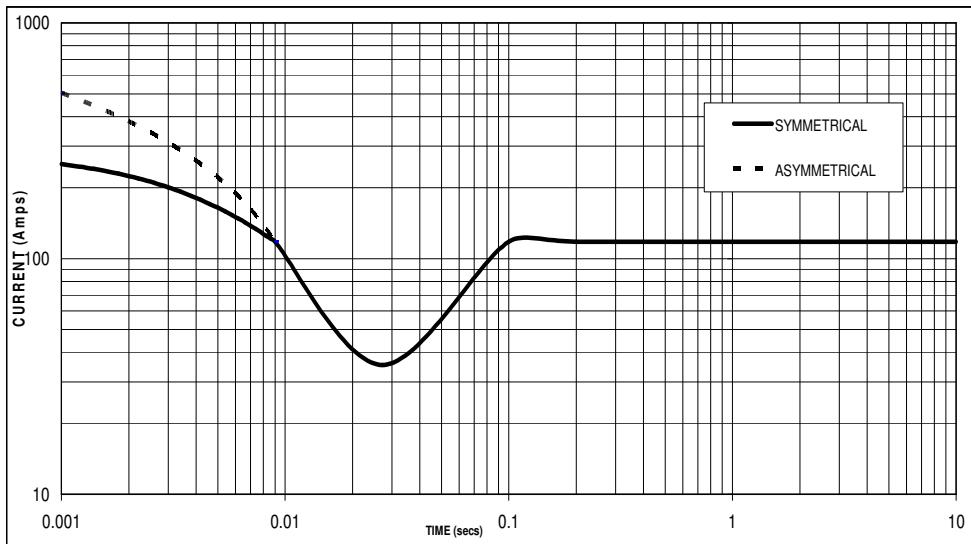
Sustained Short Circuit = 118 Amps
