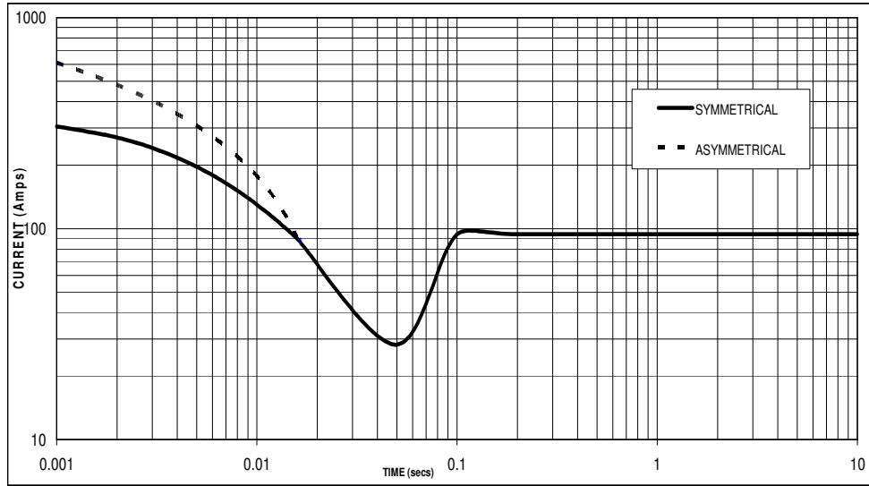
Sustained Short Circuit = 94 Amps
