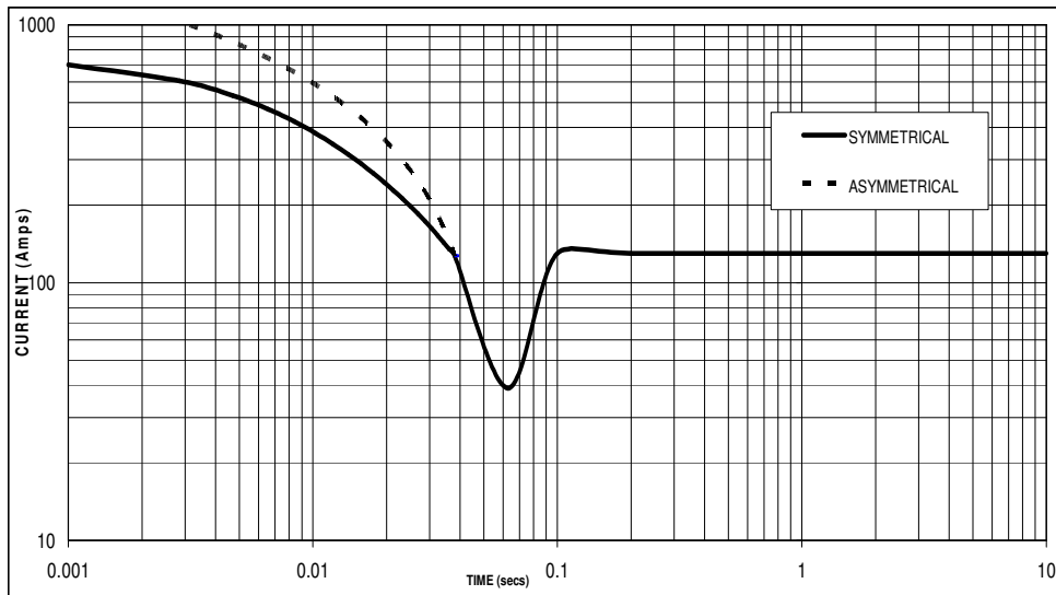
Sustained Short Circuit = 130 Amps
