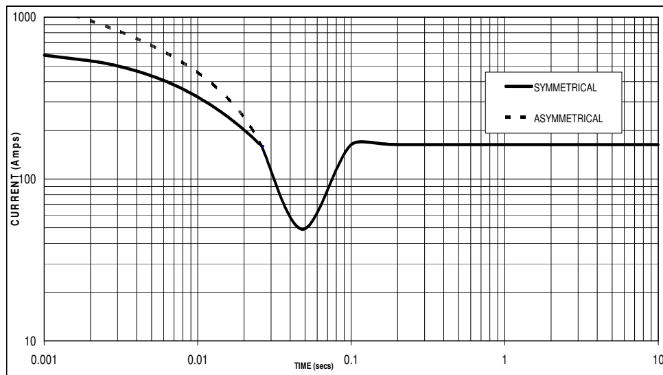
Sustained Short Circuit = 163 Amps
